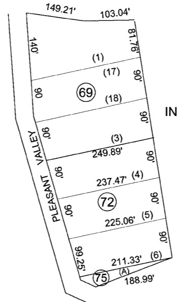
SCALE 1" = 100'
